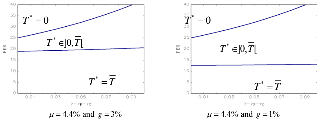
Fig 3. PER limits for the case 1 as a function of \mu - g
